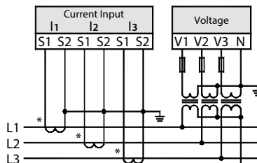
3P4W, 3CT, 3VT
