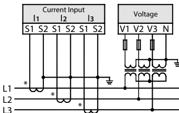
3P3W, 3CT, 3VT
