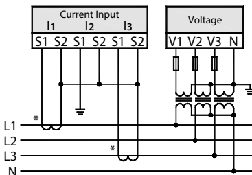
3P4W, 2CT, 3VT (for balanced 3 wire loads)
