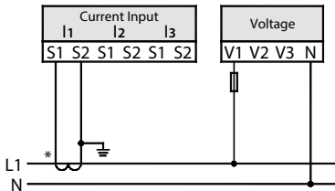
Single Phase, 1CT, no VT
