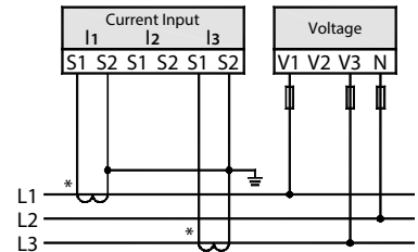
3P3W, 2CT, No VT
