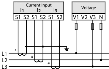
3P3W, 3CT, No VT
