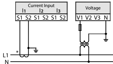
Single Phase, 1CT, VT
