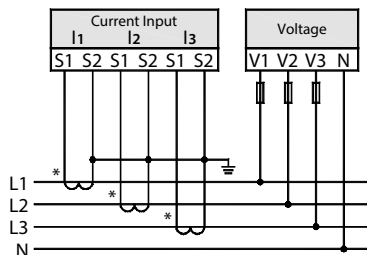
3P4W, 3CT, no VT
