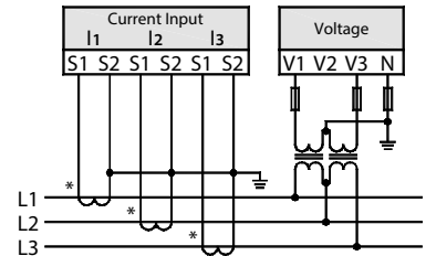
3P3W, 3CT, 2VT
