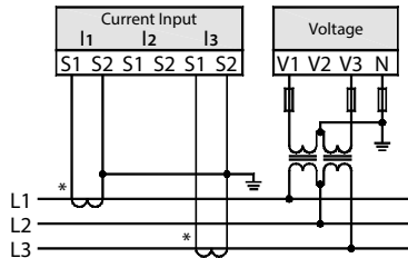
3P3W, 2CT, 2VT
